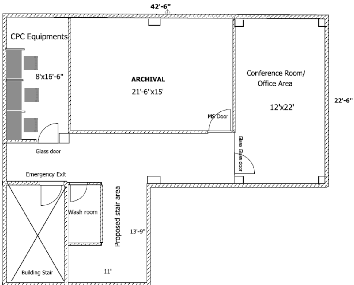
Proposed Layout Plan-2nd Floor Gujranwala Branch
