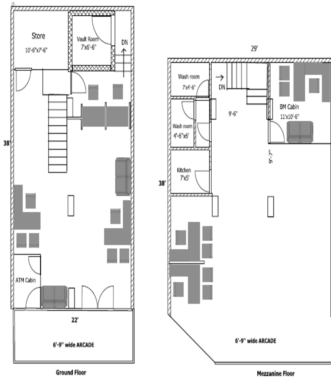
LAYOUT PLAN GULISTAN-E-JOHAR BRANCH KARACHI
